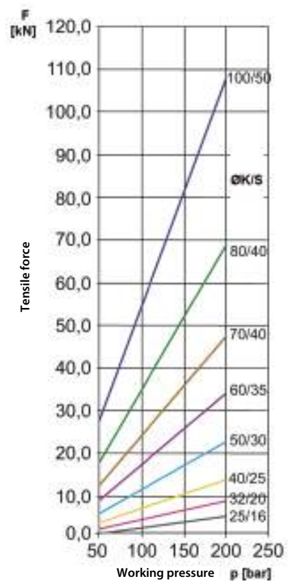
Tensile force diagram for double-acting cylinders (efficiency 92%)
